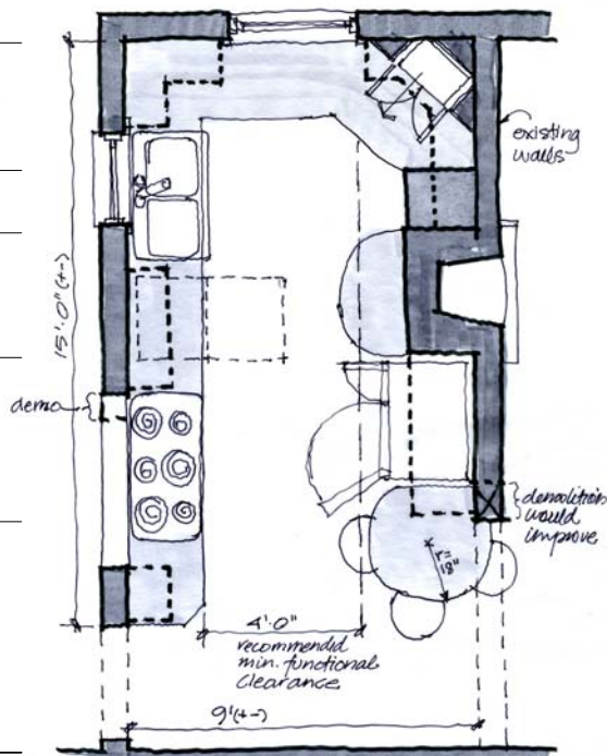
Design for People SHANTZ KITCHEN CONCEPT PLAN June 2 2015 N-7 1/2" = 1'0"
